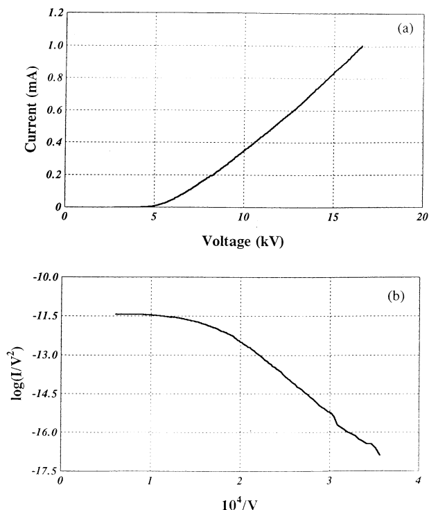
FIGURE 14. I - V characteristics showing field emission currents in the range of 0.1 nA to 1 mA. (b) Fowler-Nordheim plot corresponding to the data in (a). 47
